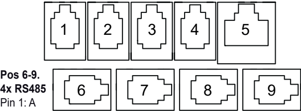
Pos 6-9. 4x RS485 Pin 1: A Pin 2: B Pin 3: 12 V Pin 4: GND
