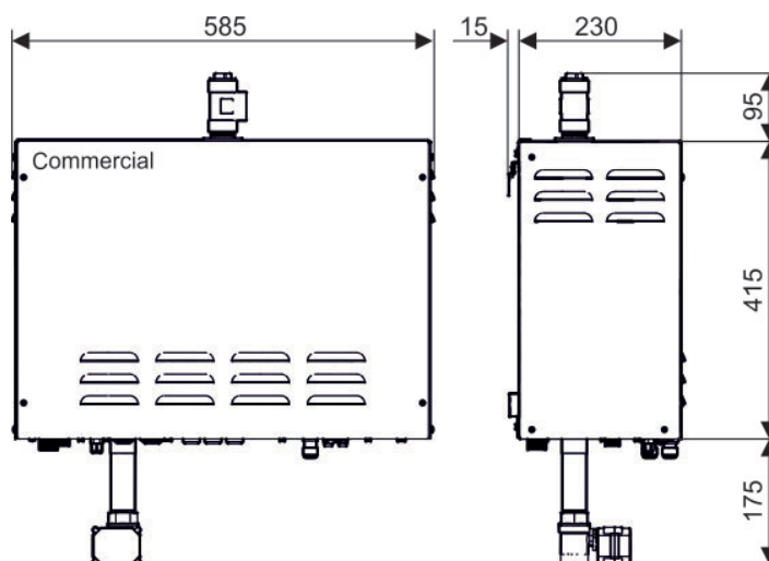
Fig. 5 Tylö Steam Generator Commercial type, dimensions in millimeters
